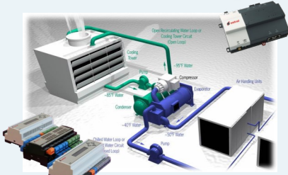
HVAC-R Control Programmable Controllers
